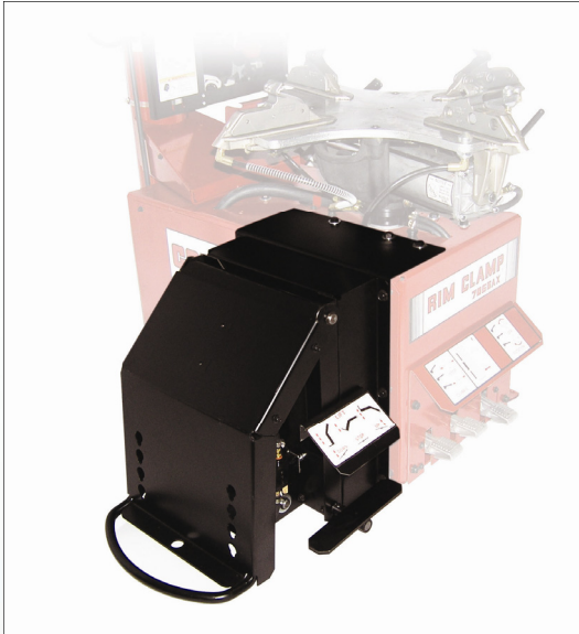
Wheel Lift System mounted on 70xx Rim Clamp
